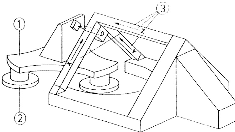
Figure 1: Scheme of the first working STM developed by Binnig, Röhrer, Gerber and Weibel at IBM Zürich in 1981. (1) Coarse approach: the 'louse' with piezoelectric base plate and three feet (2) allowing the sample to be approached towards the tip. (3) The tip is mounted on a piezoelectric tripod scanner.
