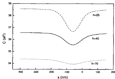
Figure 3: Calculated capacitance coupling between the S-SET and a sample with an insulating slit of width W = 100 \text{ nm} as a function of the lateral displacement x and for different tip-sample distances h . The dip in the C(x) curve is a measure of the slit by the S-SET. The graph shows that it is progressively more difficult to resolve the slit as h increases.
