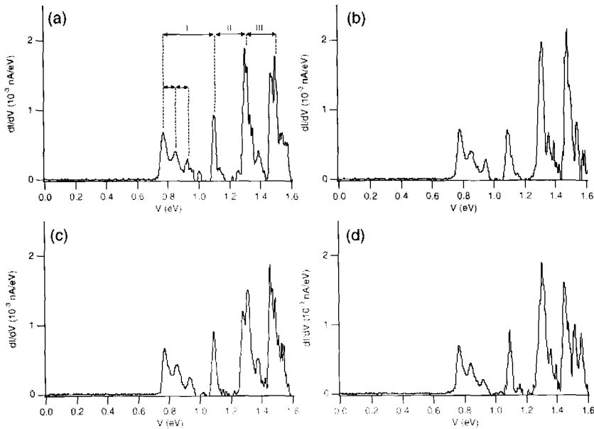
Figure 4: Tunnelling spectra measured on single CdSe clusters at 4 K for a tip-particle distance corresponding to a set-point (60 pA , 1.2 V).
