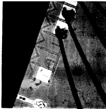
Figure 4: Picture of the S-QPC device. A row of point contacts, with different aperture widths, have been fabricated by e-beam lithography at the edge III-V heterostructure with a shallow 2DEG. The point contacts are used as electrometers in a scanning probe experiment.
